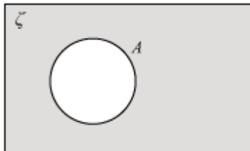
A^c (Shaded portion)
